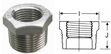
六角卜申 HEXAGON BUSHING FIG NO.9
