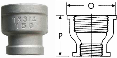
异径有边接头 REDUCEDR FIG NO.13
