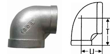
异径弯头 REDUCED ELBOW FIG NO.16
