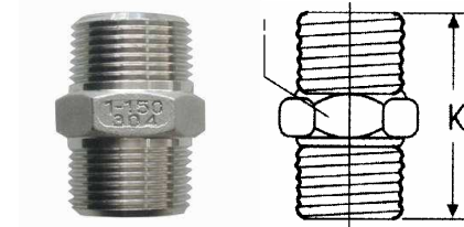
六角外牙接头 HEXAGON NIPPLE FIG NO.10
