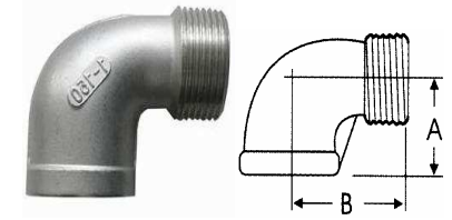
90° 内外牙弯头 90° STREET ELBOW FIG NO.4
