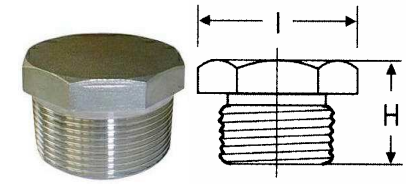
六角塞头 HEXAGON PLUG NO.8
