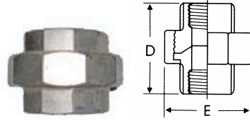
由任 UNION FIG NO.6
