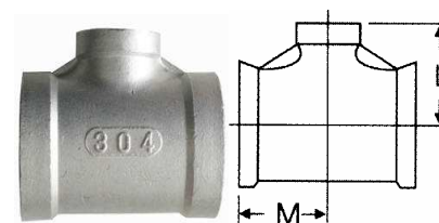
异径三通 REDUCED TEE FIG NO.11
